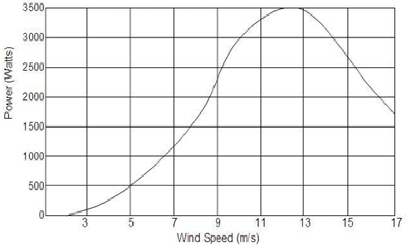
CWE-FRE-3KW Power Curve
